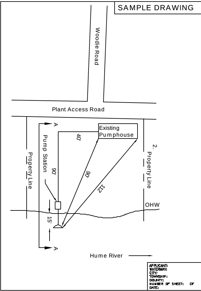
Intake/Outfall Structures
