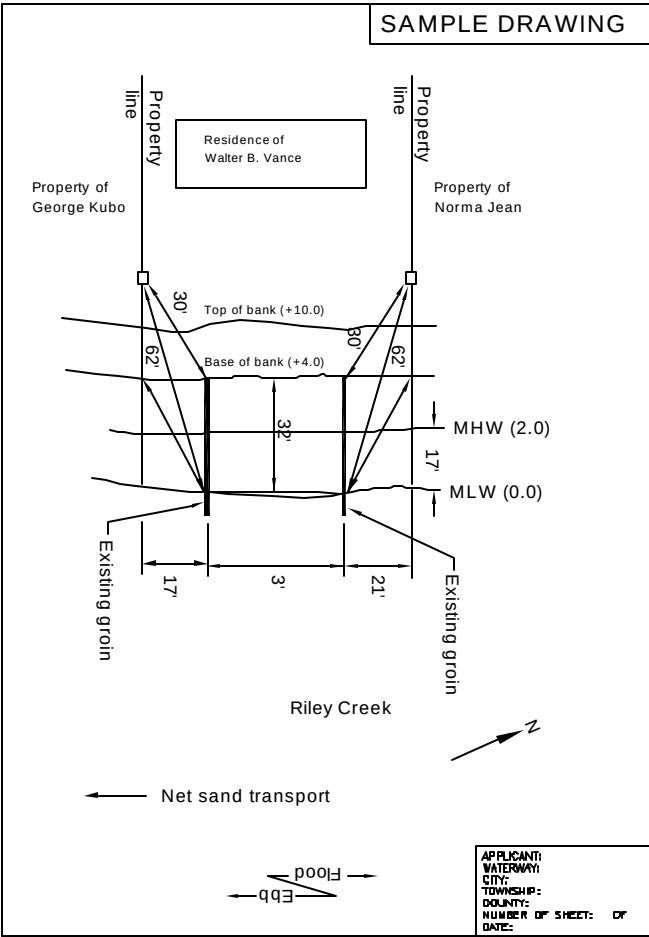
Beach Nourishment
